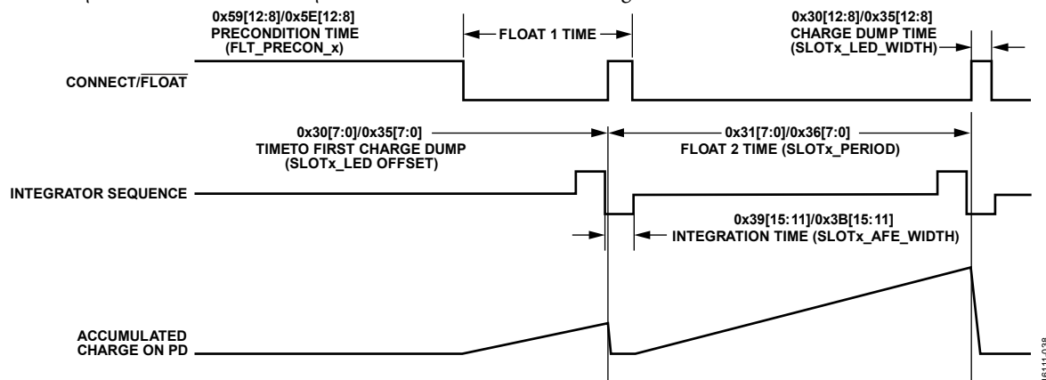
Figure 38. Example of Float Ambient Mode Timing
