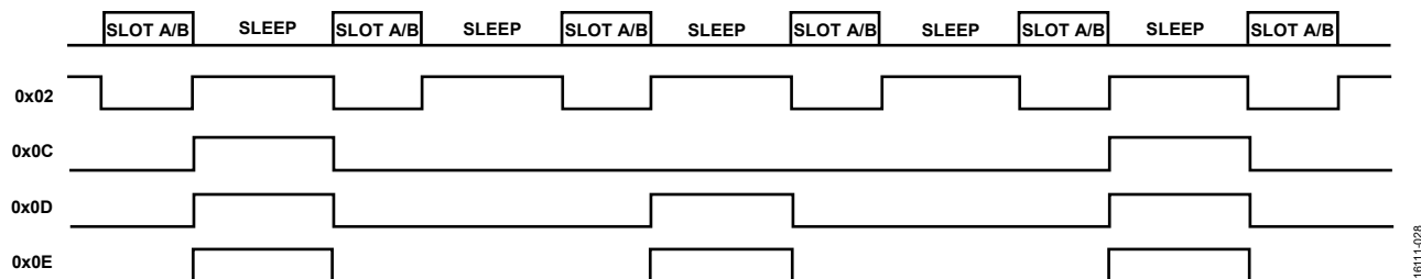
Figure 28. Optional Timing Signals Available on GPIOx—Register 0x0B, Bits[12:8] or Bits[4:0] = 0x02, 0x0C, 0x0D, and 0x0E
