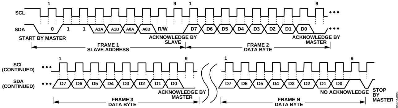
Figure 17. General I²C Read Timing Diagram
