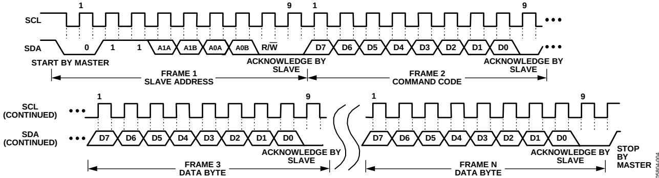
Figure 16. General I²C Write Timing Diagram
