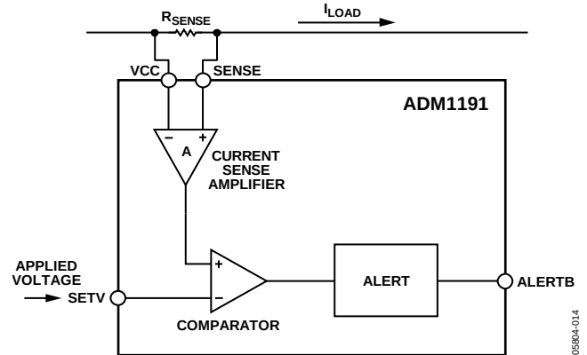
Figure 26. SETV Operation
