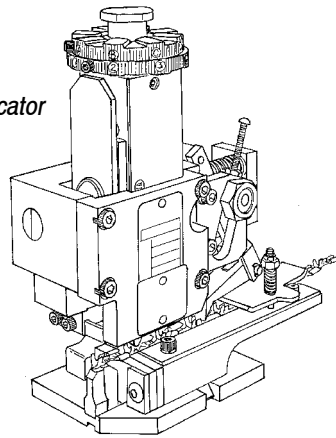
Typical HDM Quick-Change Applicator (Side-Feed Type)
