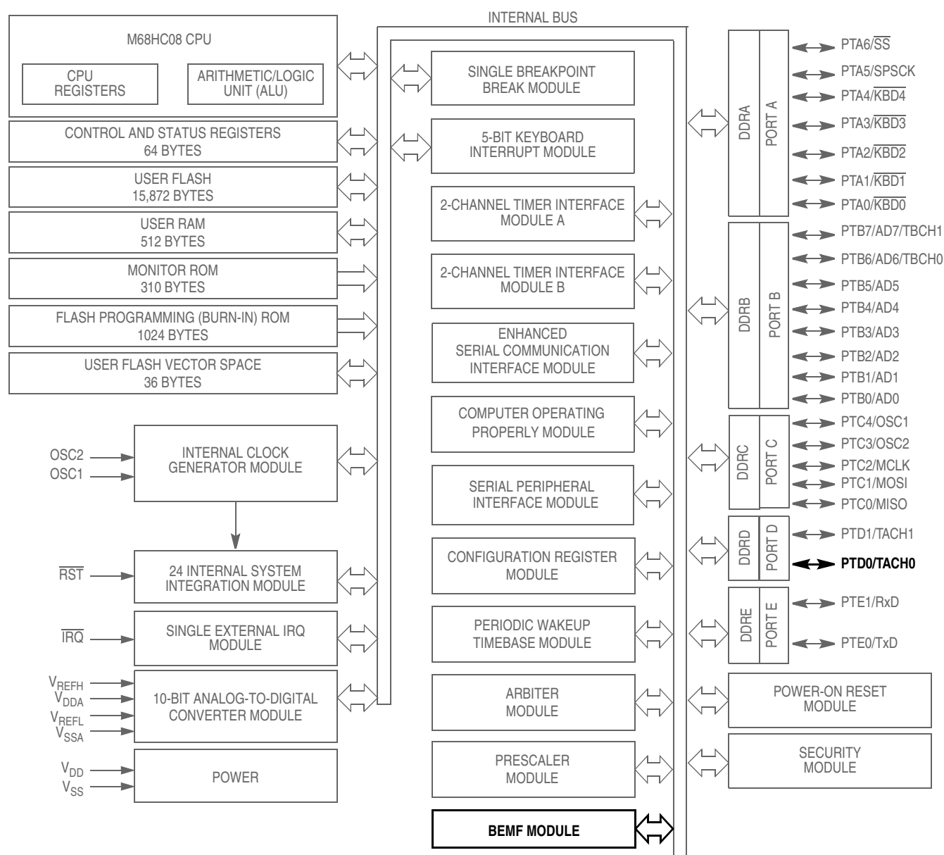
Figure 4-2. Block Diagram Highlighting BEMF Block and Pins
