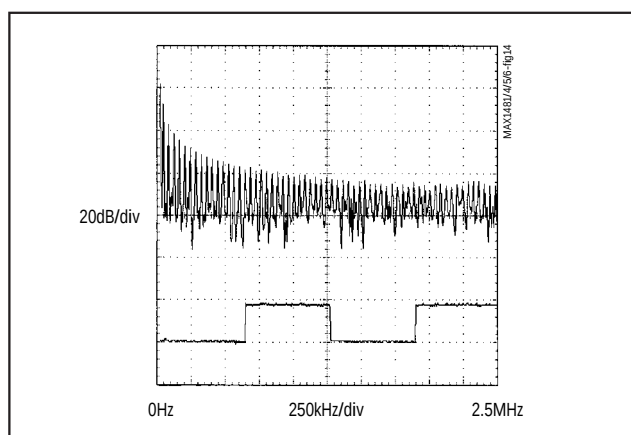
Figure 14. Driver Output Waveform and FFT Plot of MAX1484/MAX1486 Transmitting a 20kHz signal
