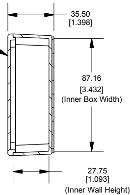
SECTION A-A End View of Assembly
