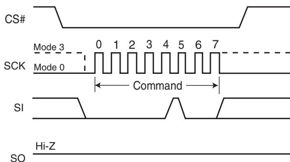
Figure 9.6 Write Disable (WRDI) Command Sequence
