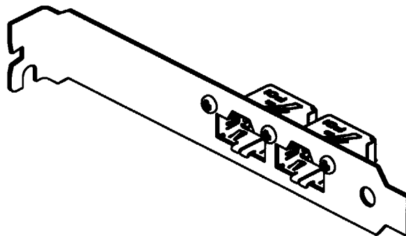
TWO POSITION(P/N 73592-002 or -006) SCALE 4:5
