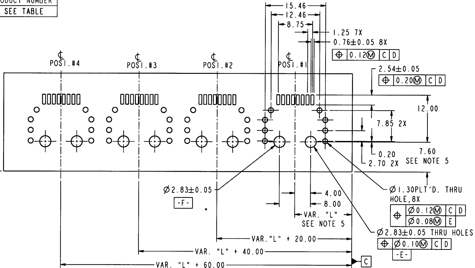
RECOMMENDED PCB LAYOUT (AS VIEWED FROM COMPONENT SIDE) SCALE 9:5
