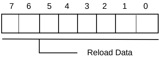
Figure 51. Timer Reload Register Channel 1H
