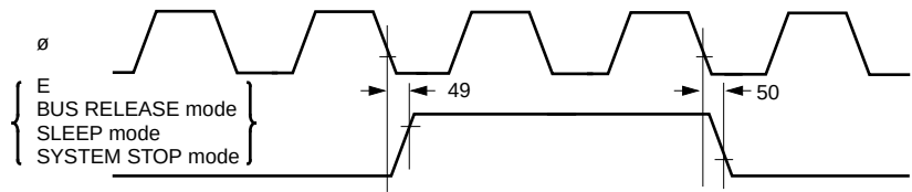
Figure 25. \overline{E} Clock Timing (BUS RELEASE Mode, SLEEP Mode, SYSTEM STOP Mode)
