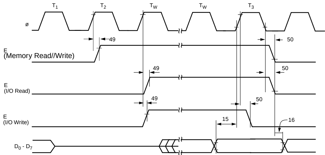
Figure 24. \overline{E} Clock Timing (Memory Read/Write Cycle, I/O Read/Write Cycle)
