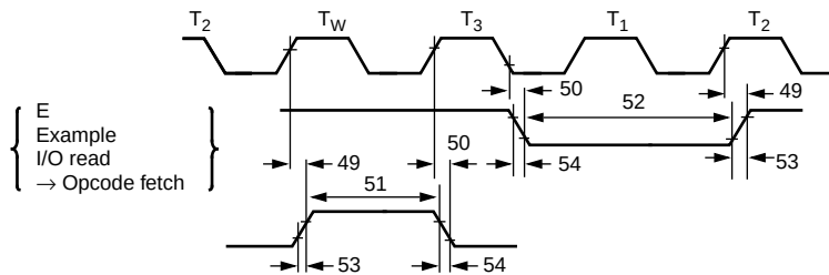
Figure 26. \overline{E} Clock Timing (Minimum timing example of P_{WEL} and P_{WEH} )
