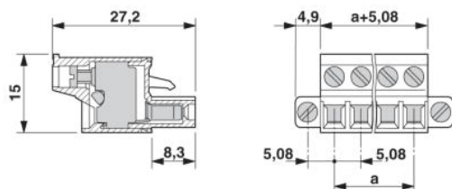
Dimensioned drawing
