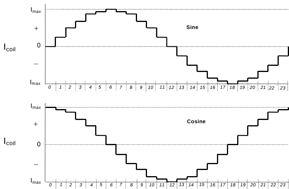
Figure 6. Microstepping
