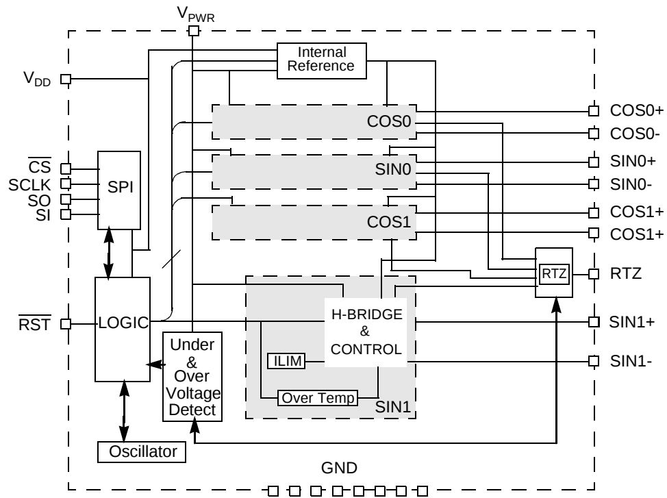
Figure 1. 33991 Block Diagram
