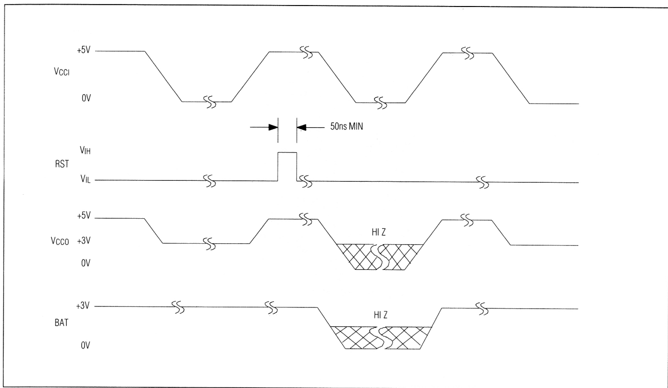
Figure 4. Reset Timing
