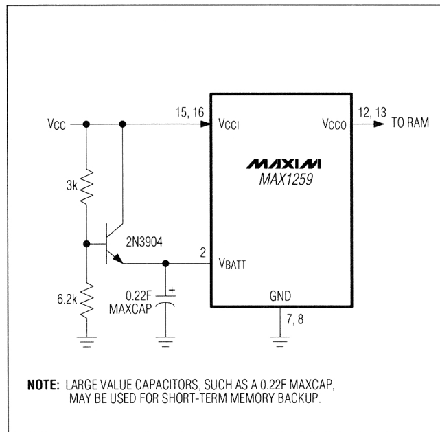
Figure 3. Using a MAXCAP as a Backup Battery
