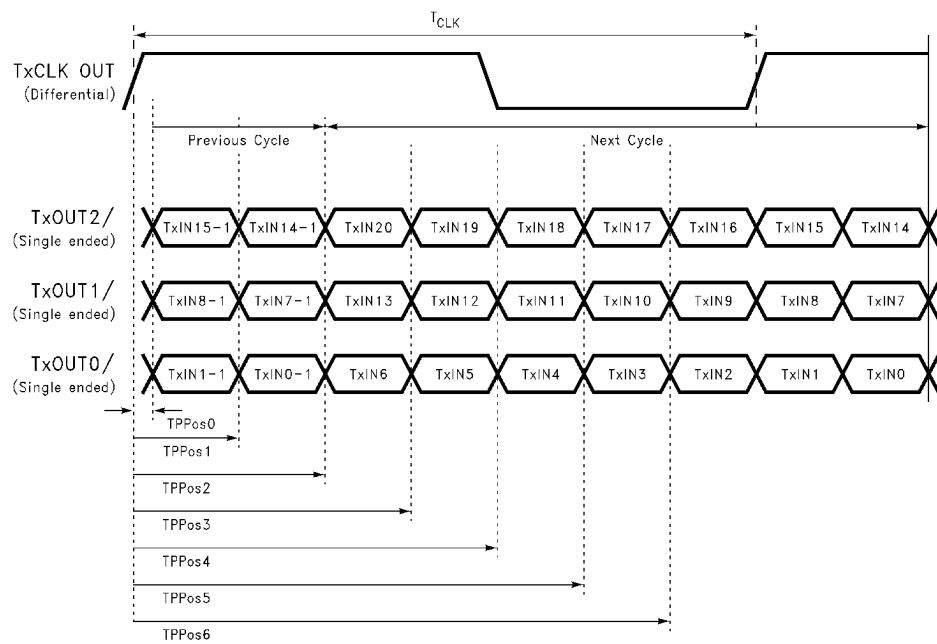
FIGURE 16. Transmitter LVDS Output Pulse Position Measurement
