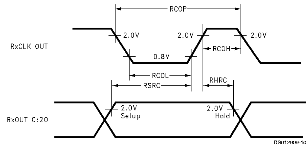
FIGURE 7. D590CR216 (Receiver) Setup/Hold and High/Low Times
