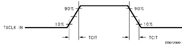
FIGURE 4. D590CR215 (Transmitter) Input Clock Transition Time
