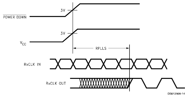
FIGURE 11. DS9OCR216 (Receiver) Phase Lock Loop Set Time
