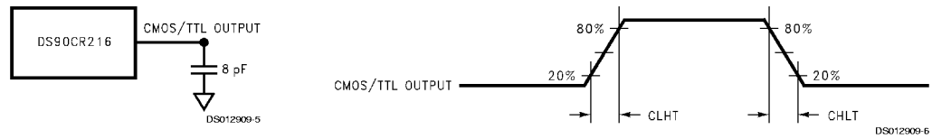
FIGURE 3. DS90CR216 (Receiver) CMOS/TTL Output Load and Transition Times
