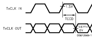
FIGURE 8. DS90CR215 (Transmitter) Clock In to Clock Out Delay
