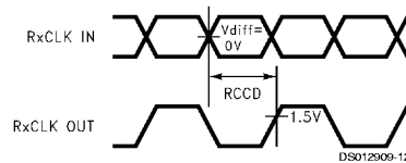
FIGURE 9. D590CR216 (Receiver) Clock In to Clock Out Delay
