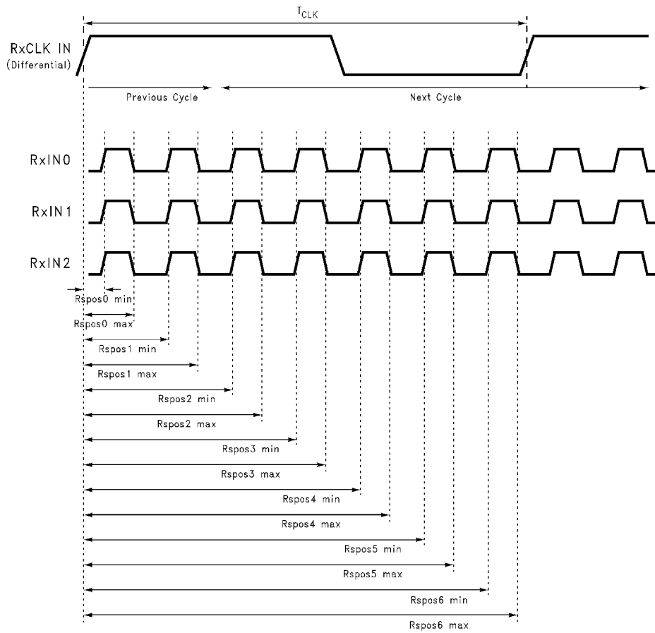
FIGURE 17. Receiver LVDS Input Strobe Position
