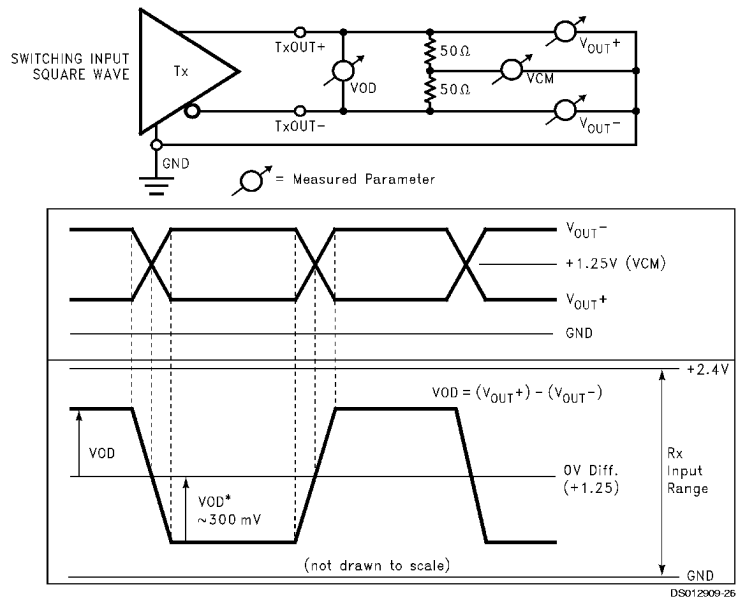
FIGURE 21. Single-Ended and Differential Waveforms
