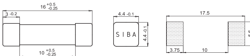
Recommended Pad Layout
