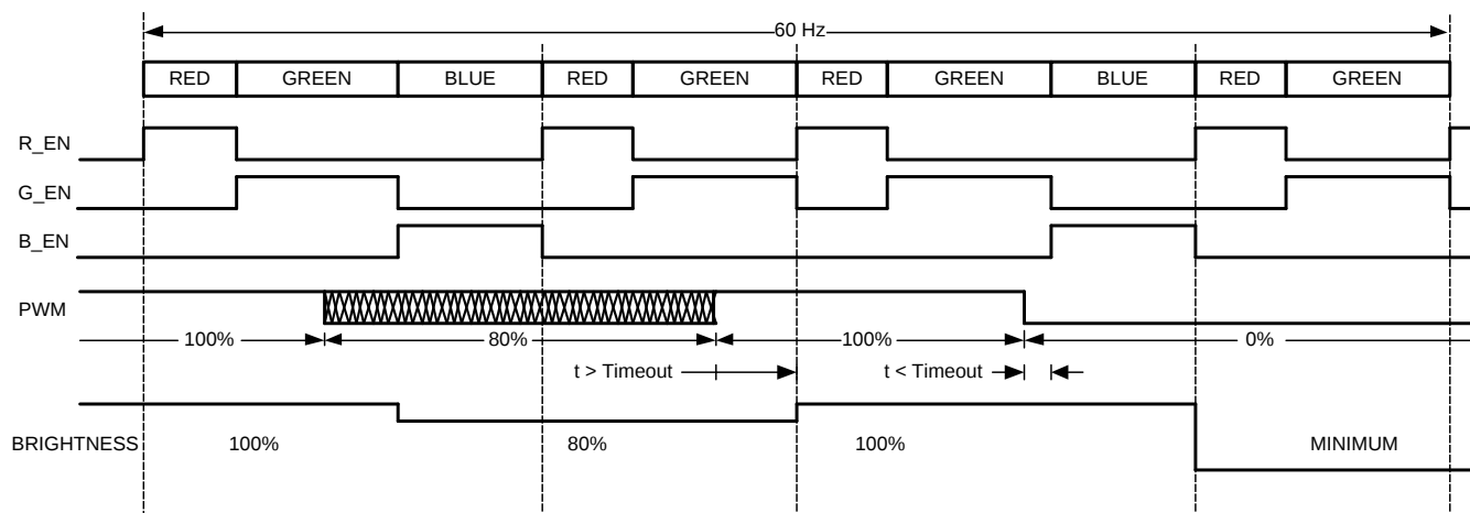
Figure 18. PWM Timing
