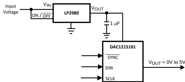
Figure 44. Using the LP2980 regulator
