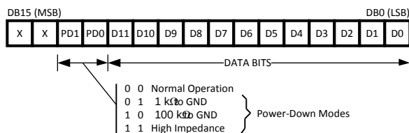
Figure 36. Input Register Contents
