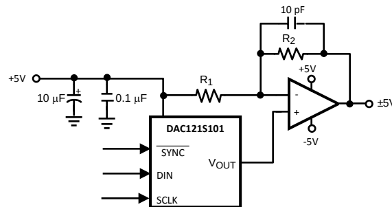
Figure 45. Bipolar Operation
