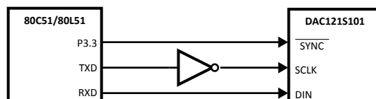
Figure 38. 80C51/80L51 Interface
