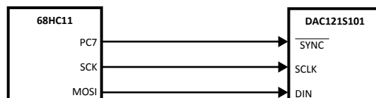
Figure 39. 68HC11 Interface
