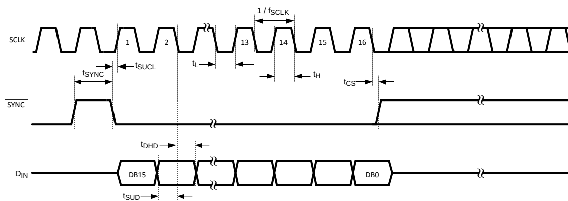
Figure 2. DAC121S101 Timing
