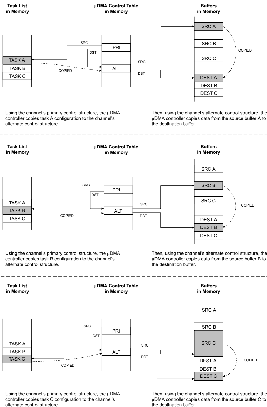
Figure 8-4. Memory Scatter-Gather, \mu DMA Copy Sequence
