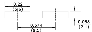
Recommended land pattern
