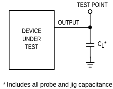
Figure 2. Test Circuit
