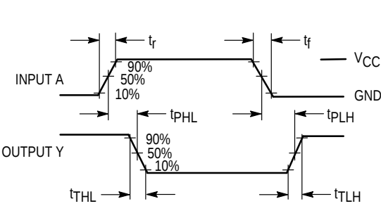
Figure 1. Switching Waveforms
