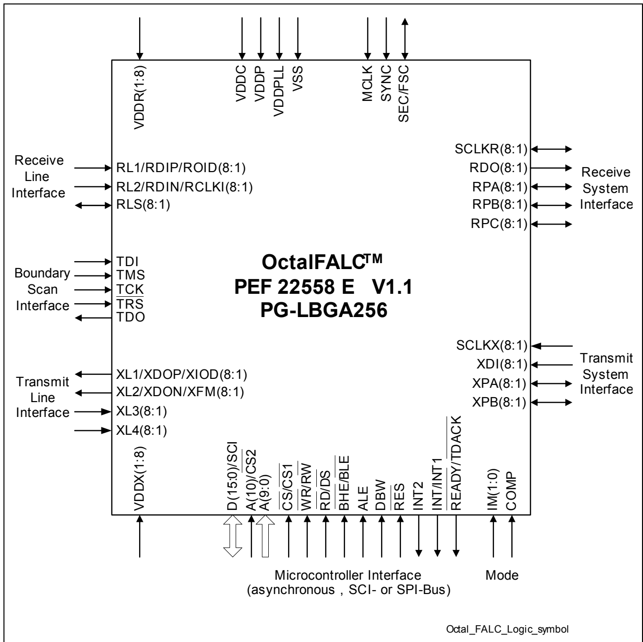
Figure 1 Logic Symbol
