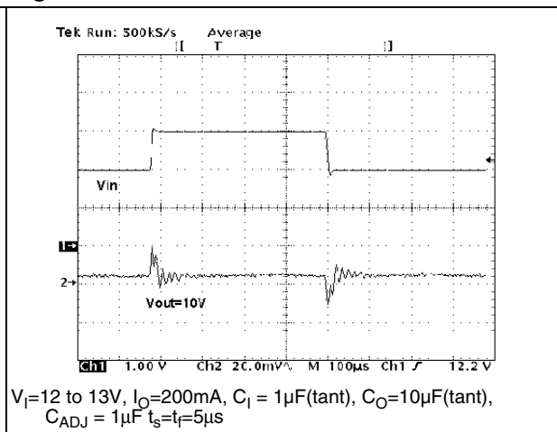
Figure 30. Line transient
