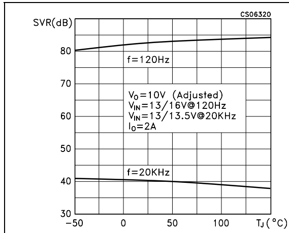
Figure 23. Stability
