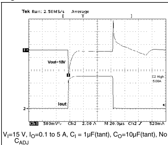
Figure 31. Load Transient
