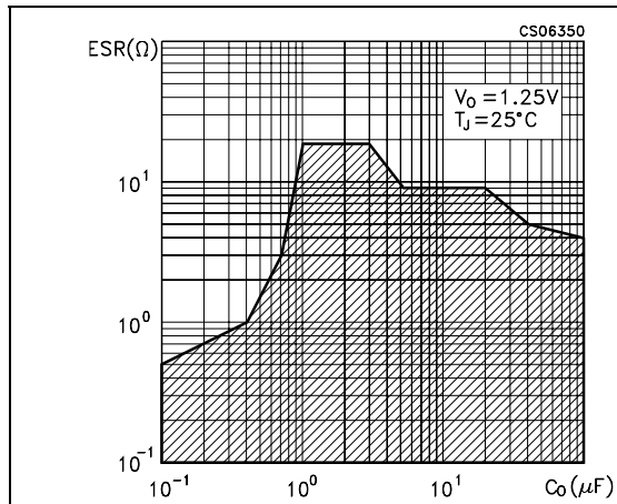
Figure 25. Stability
