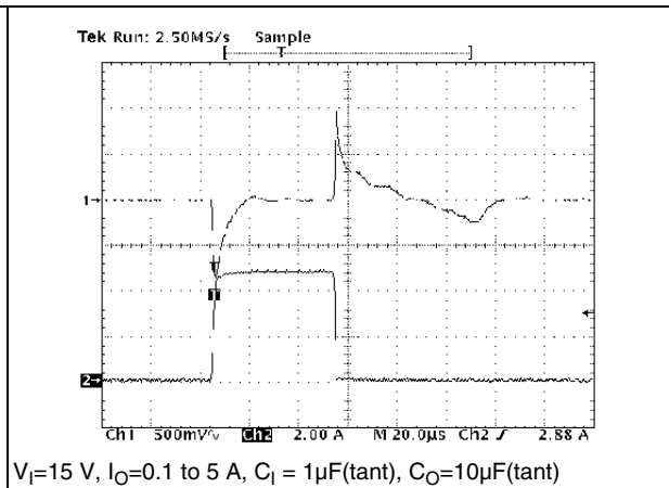
Figure 28. Load transient
