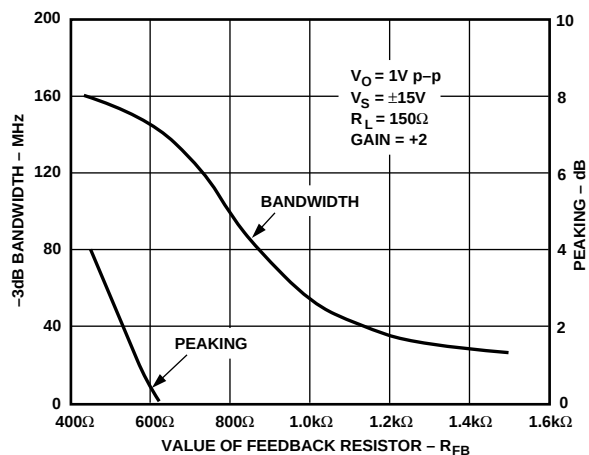
Figure 12. 3 dB Bandwidth & Peaking vs. Value of R_{FB}
