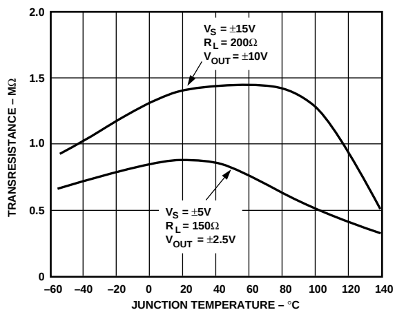
Figure 8. Transresistance vs. Junction Temperature
