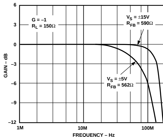
Figure 26. Closed-Loop Gain vs. Frequency, Gain = -1
