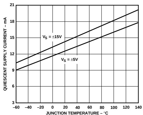
Figure 4. Quiescent Supply Current vs. Junction Temperature
