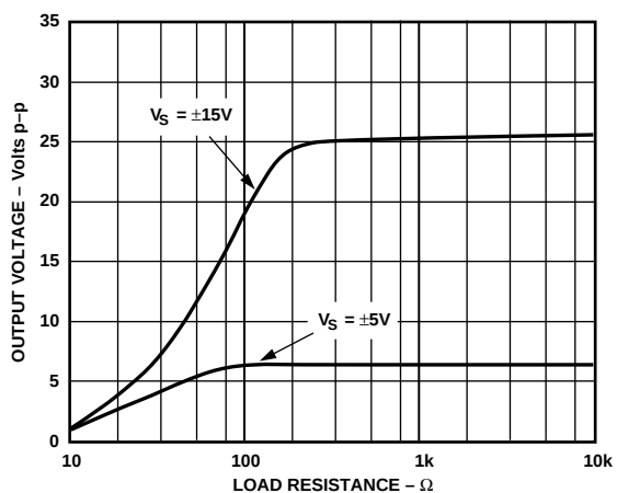
Figure 3. Output Voltage Swing vs. Resistive Load
