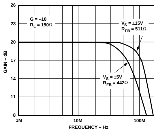
Figure 28. Closed-Loop Gain vs. Frequency, Gain = -10
