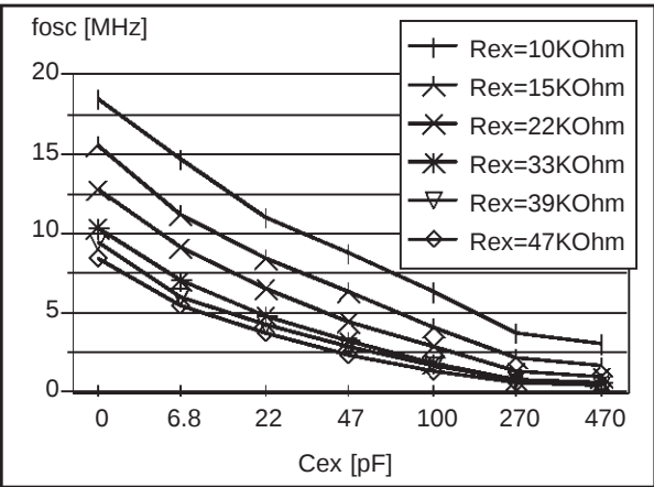
Figure 67. Typical External RC Oscillator
