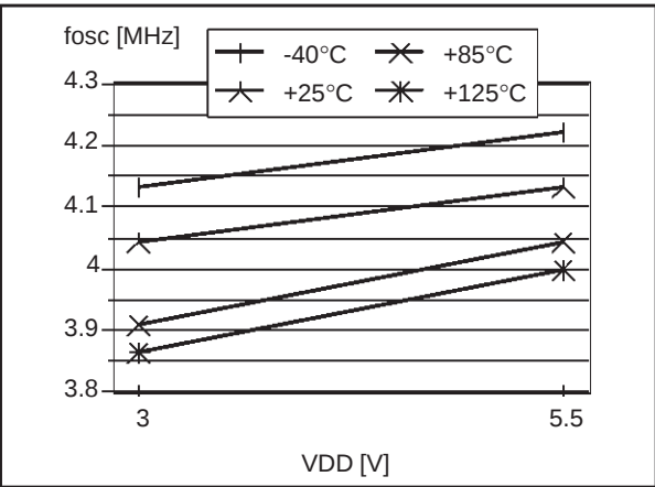
Figure 66. Typical Internal RC Oscillator
