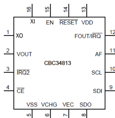
Figure 1: CBC34813 Pin-out Diagram
