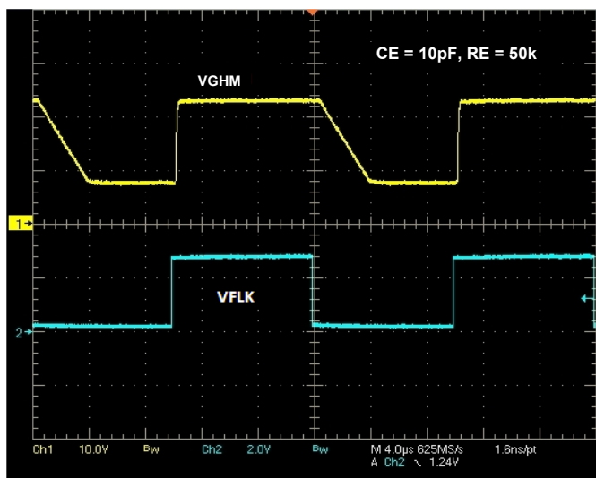
FIGURE 7. GPM CIRCUIT WAVEFORM
