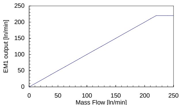
Figure 2: Typical CMOSens® EM1 Mass Flow Meter transfer characteristics.
