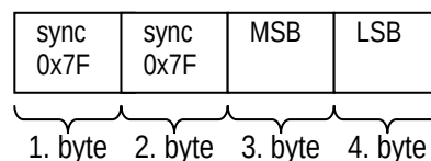
Figure 7: Byte sequence of one value
