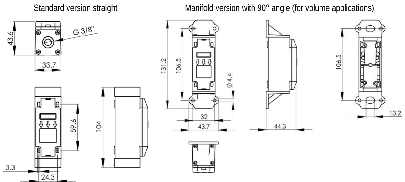
Figure 8: Physical dimensions and mounting information of the CMOSens® EM1. All units are in [mm]
