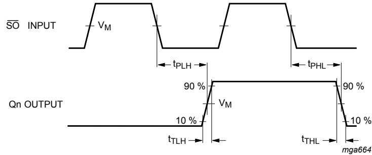
Fig. 9. Propagation delay \overline{S\overline{O}} input to Qn outputs and the output transition time
