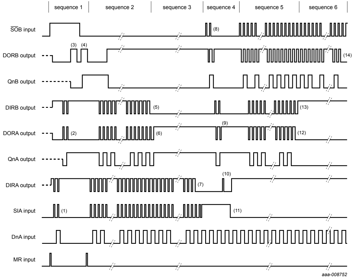
Fig. 23. Waveforms showing the functionality and intercommunication between to FIFOs
