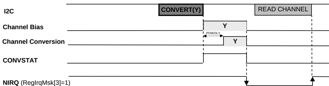
Figure 20 – Manual Mode – CONVERT Command (CHAN = Y; PROXSCANPERIOD = 0)
