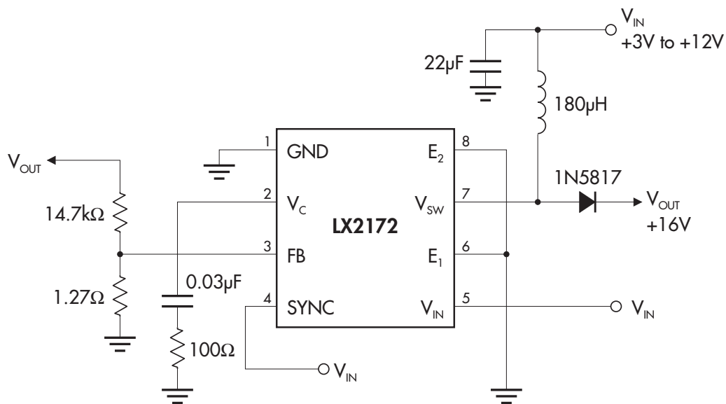
FIGURE 1 — Boost Coverter Circuit Using The LX2172 / 2173
