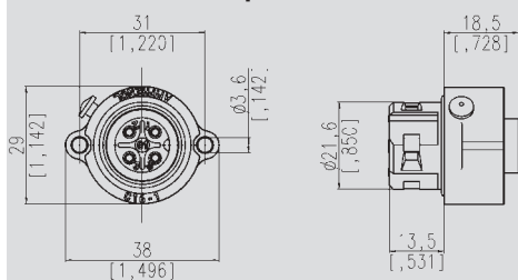
Female Receptacle
