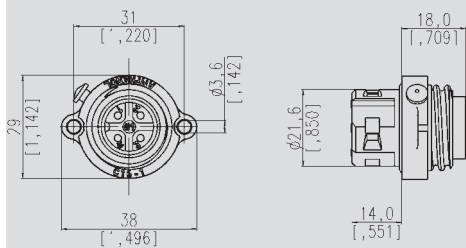
Male Receptacle
