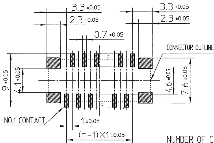
RECOMMENDED PC BOARD LAYOUT (COMPONENT SIDE)
