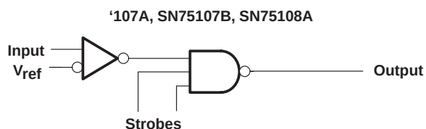
Figure 13. Single-Ended Operation
