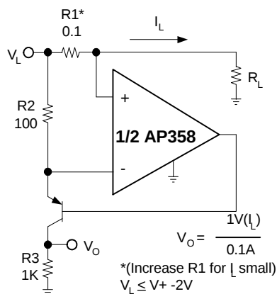
Current Monitor
