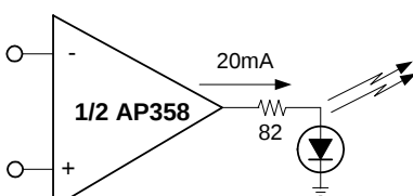
LED Driver
