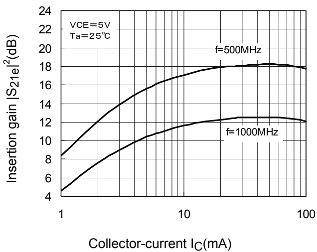
|S_{21e}|^2-I_C
