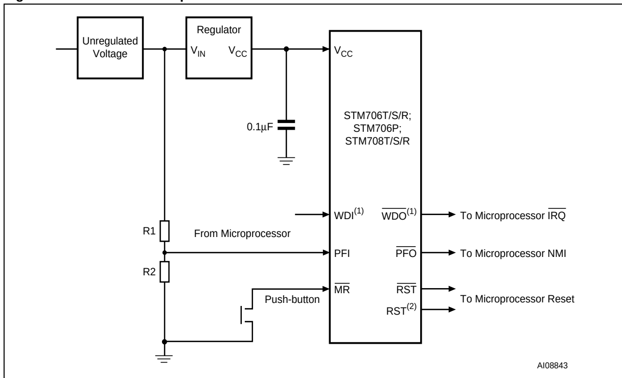
Figure 10. Hardware Hookup
