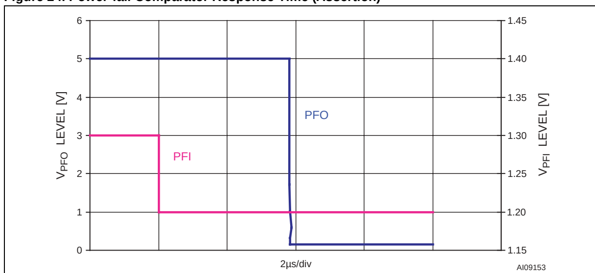
Figure 24. Power-fail Comparator Response Time (Assertion)
