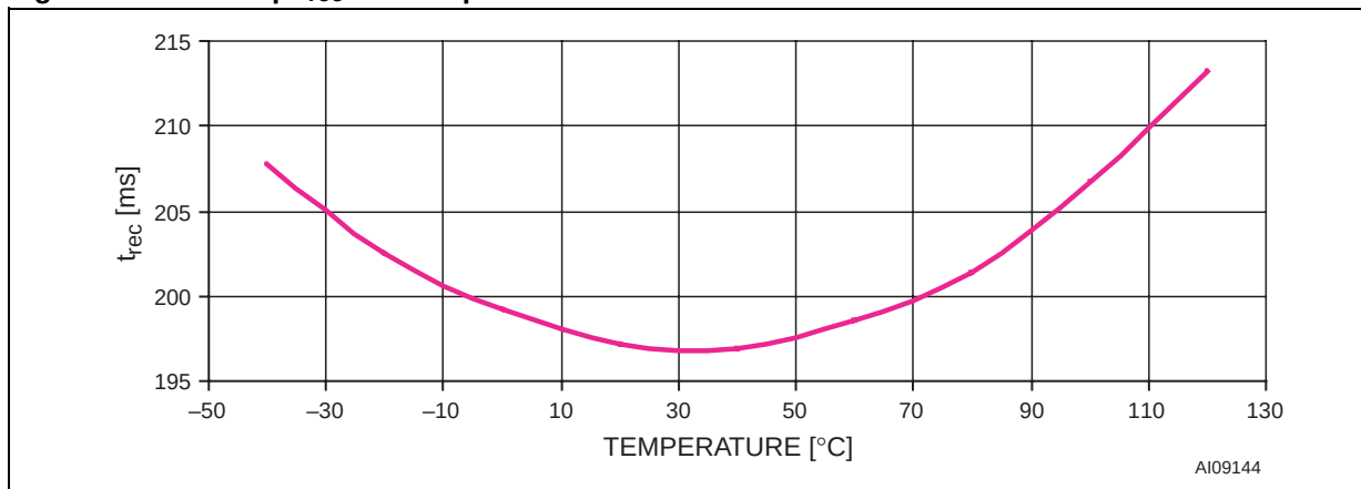
Figure 16. Power-up t_{rec} vs. Temperature
