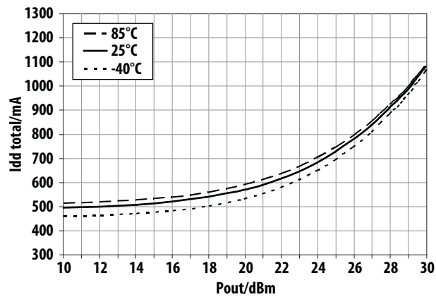
Figure 10. Over-temperature I_{dd\_total} vs P_{out} @ 2.6GHz
