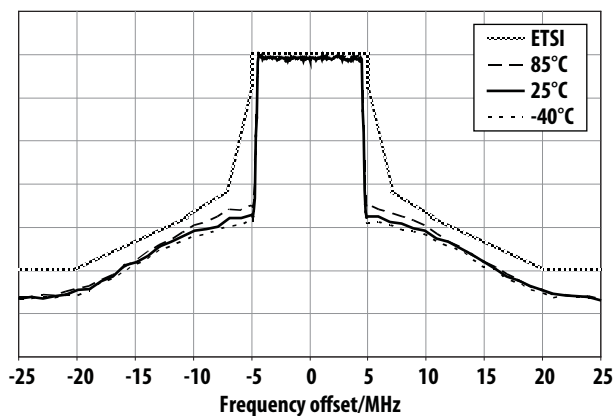
Figure 33. Over-temperature ETSI SEM at 26.5dBm Pout @ 2.6GHz
