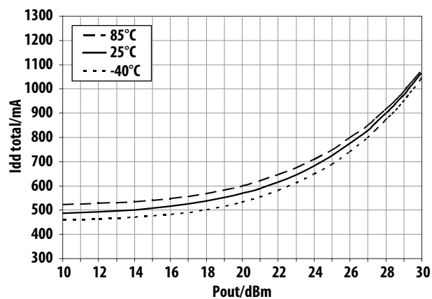
Figure 8. Over-temperature I_{dd\_total} vs P_{out} @ 2.5GHz
