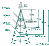
Hi-Spot 95 75W/30°
