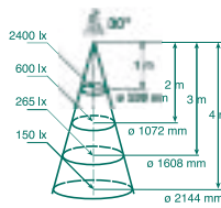
Hi-Spot 120 75W/30°
