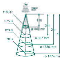
Hi-Spot 95 75W/30°
