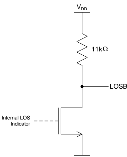
FIGURE 7. LOSB EQUIVALENT OUTPUT STRUCTURE
