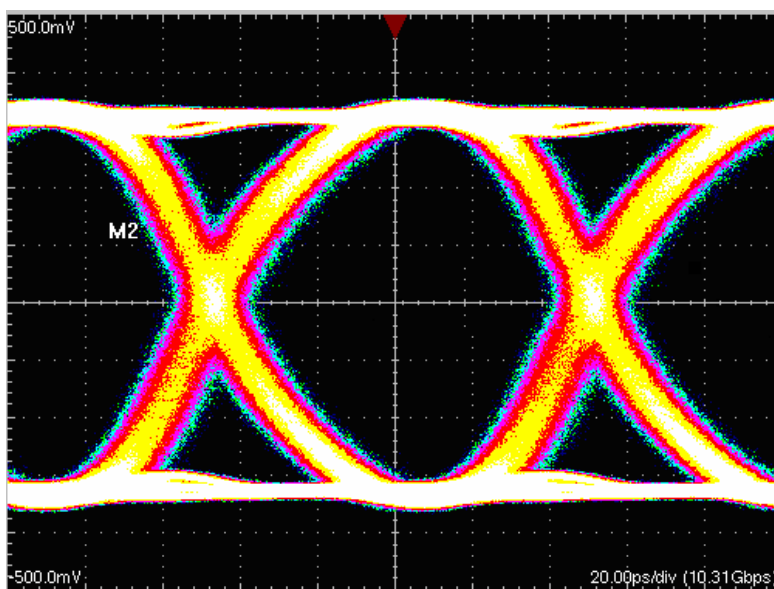
FIGURE 3. ISL36111 10.3125Gb/s OUTPUT FOR A 10M 28AWG CABLE
