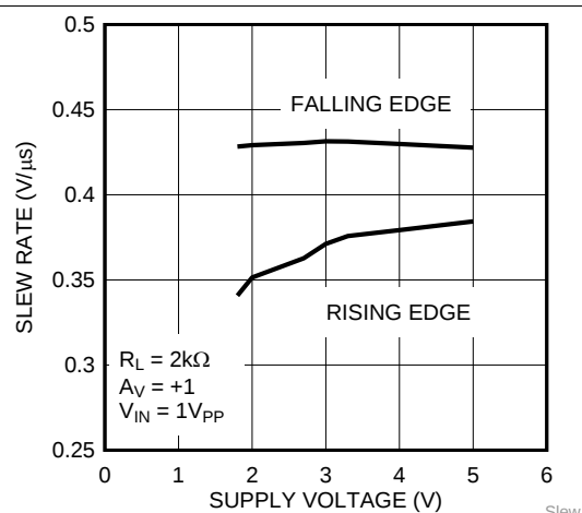
Figure 20. Slew Rate vs Supply Voltage LMV612 Only
