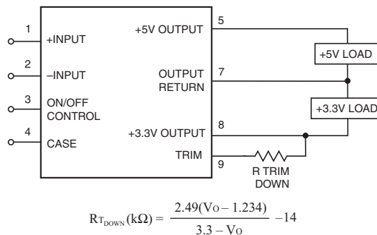
Figure 4. Decrease Output Voltage Trim Connections Using A Fixed Resistor
