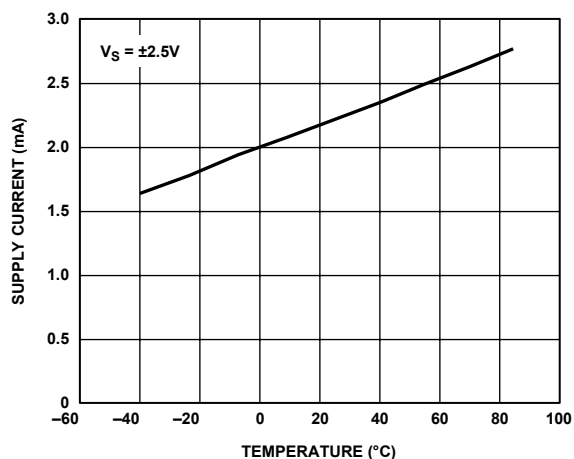
Figure 45. Supply Current vs. Temperature
