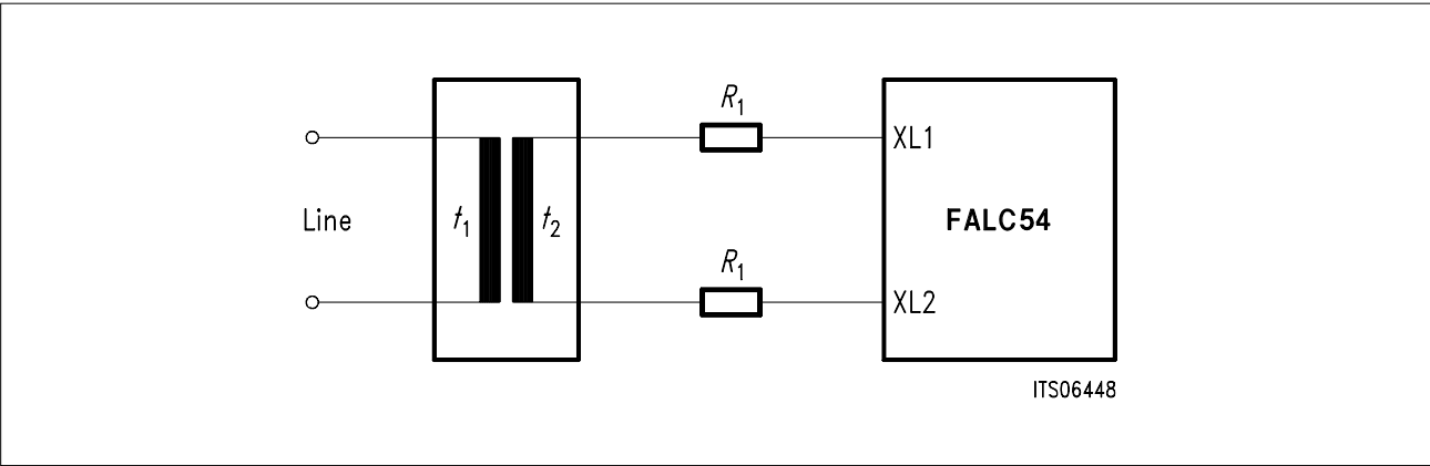
Figure 47 Transmitter Configuration
