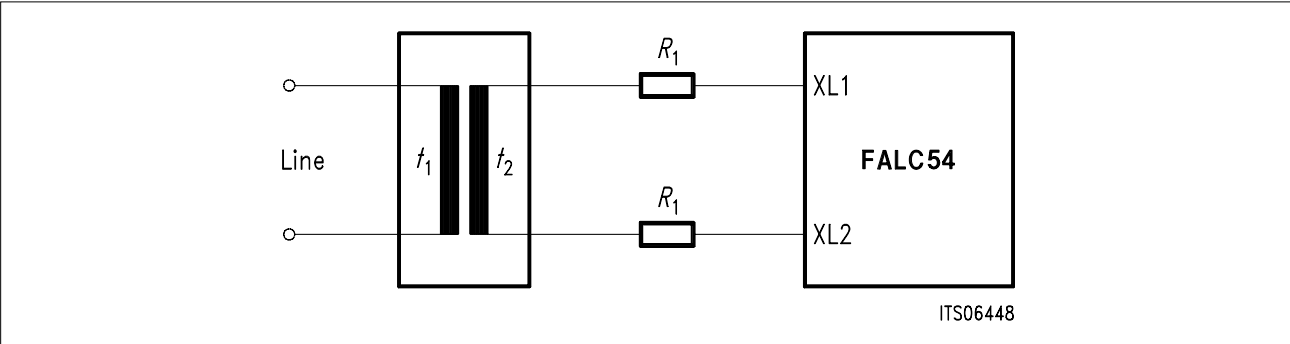
Figure 15 Transmitter Configuration
