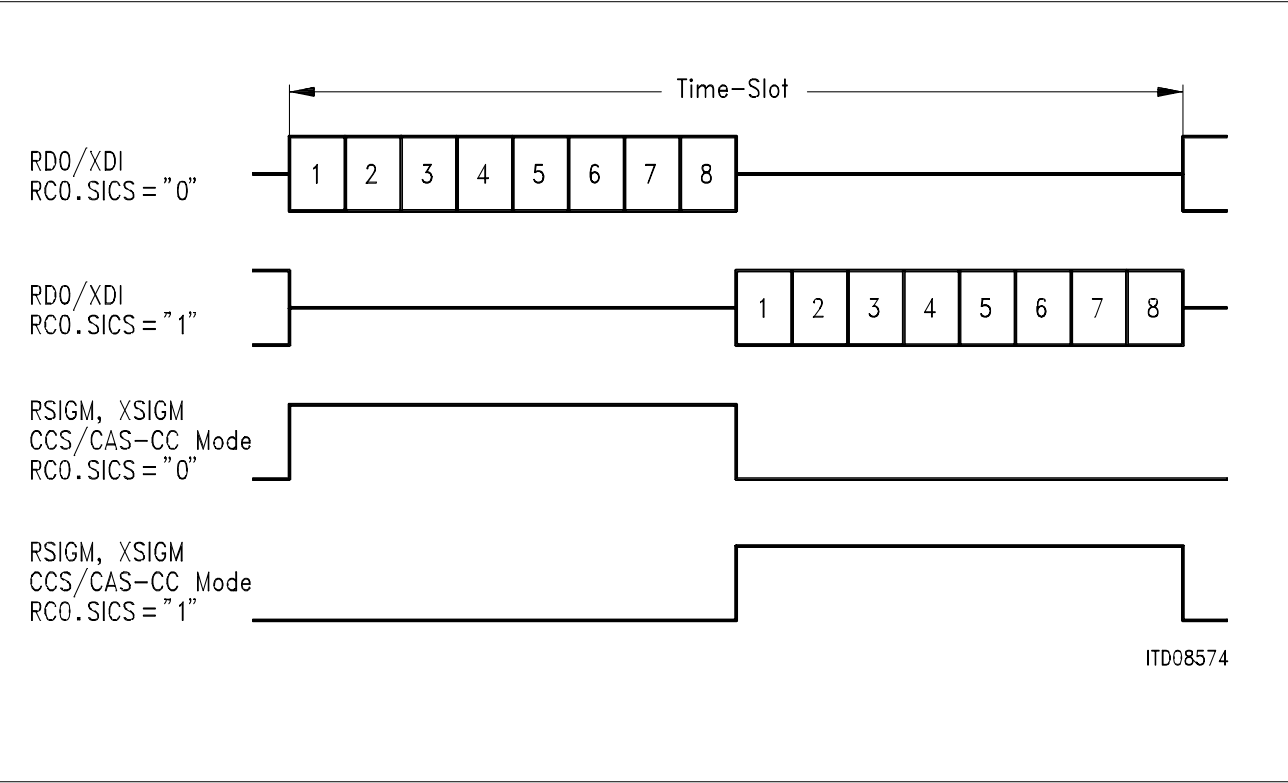
Figure 29 4-Mbyte System Interface Mode
