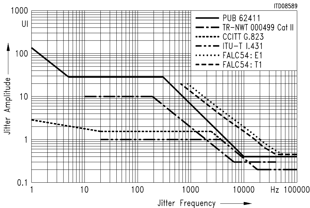
Figure 12 Jitter Tolerance
