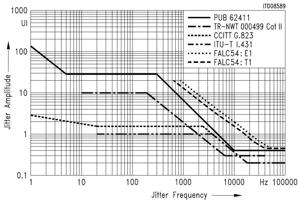
Figure 44 Jitter Tolerance
