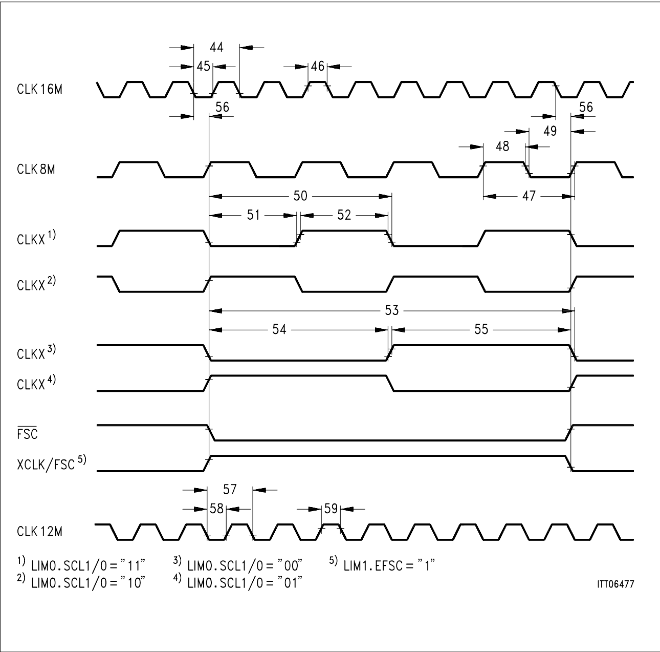
Figure 79 Timing of the System Clock Interface
