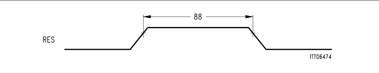
Figure 84 Reset Timing
