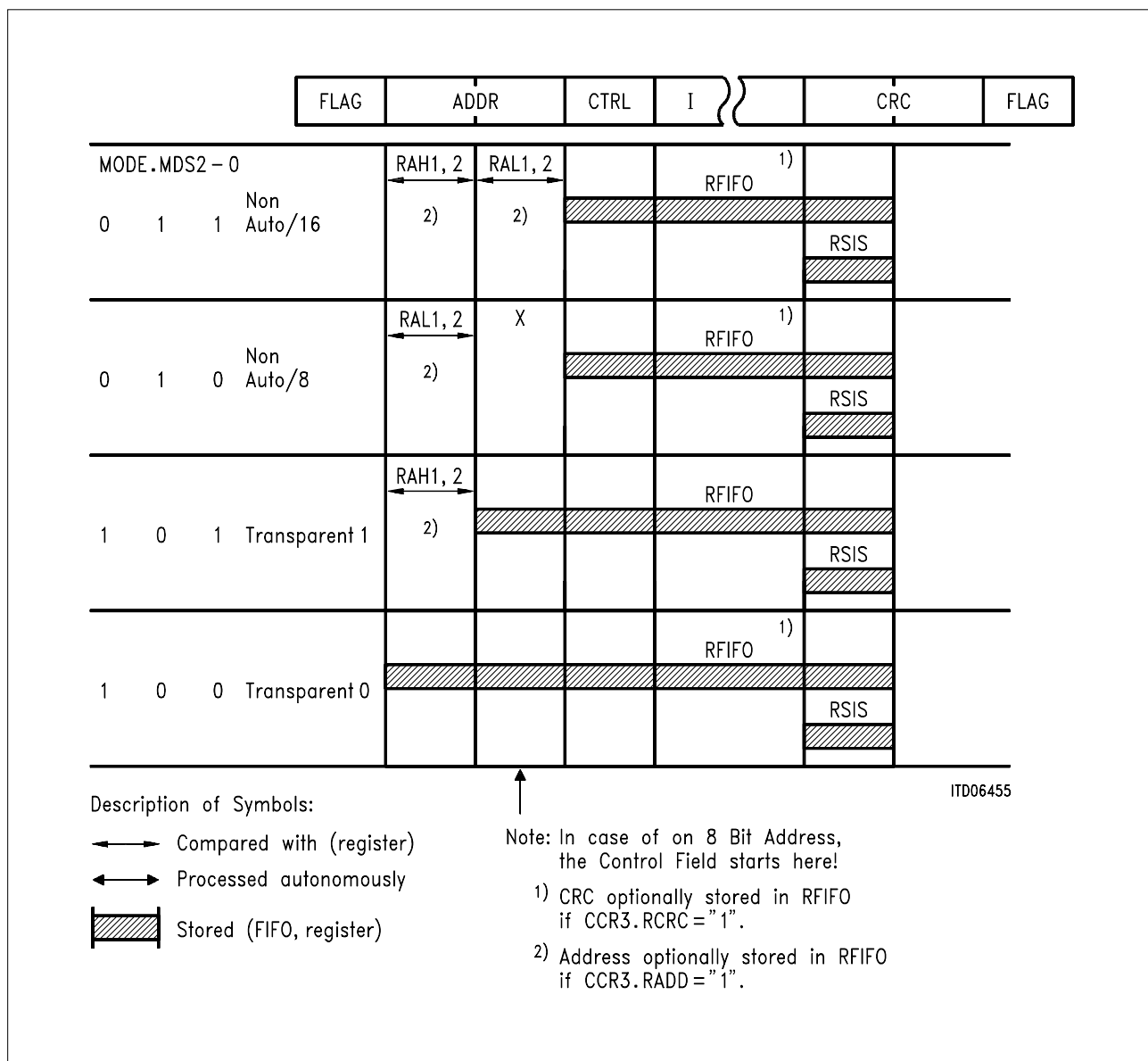
Figure 54 Receive Data Flow of FALC
