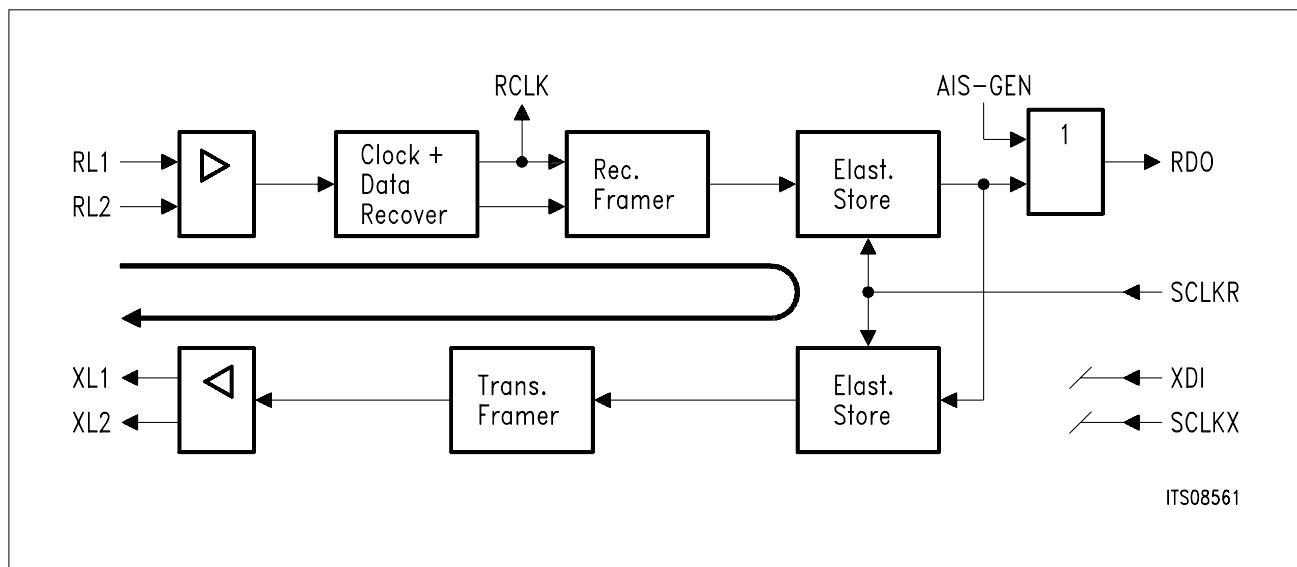
Figure 50 Payload Loop
