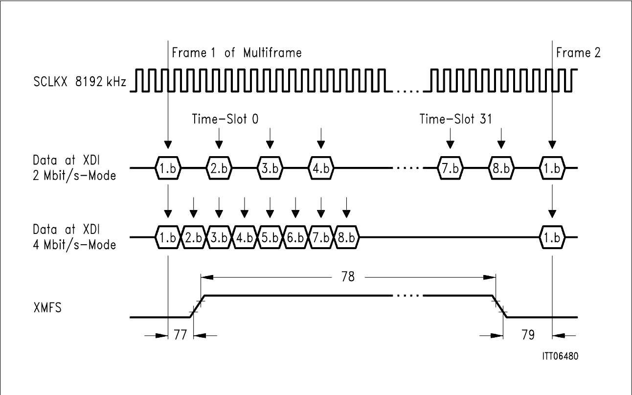
Figure 82 XMFS-Timing
