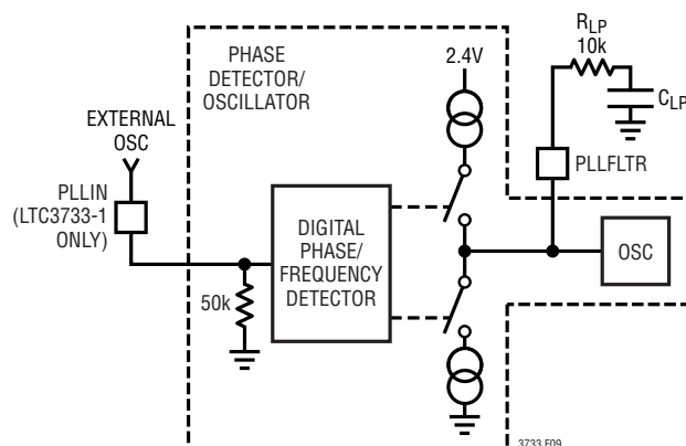
Figure 9. Phase-Locked Loop Block Diagram
