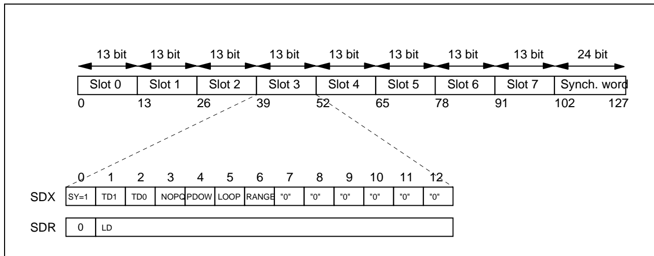
Figure 9 Frame Structure on SDX and SDR
