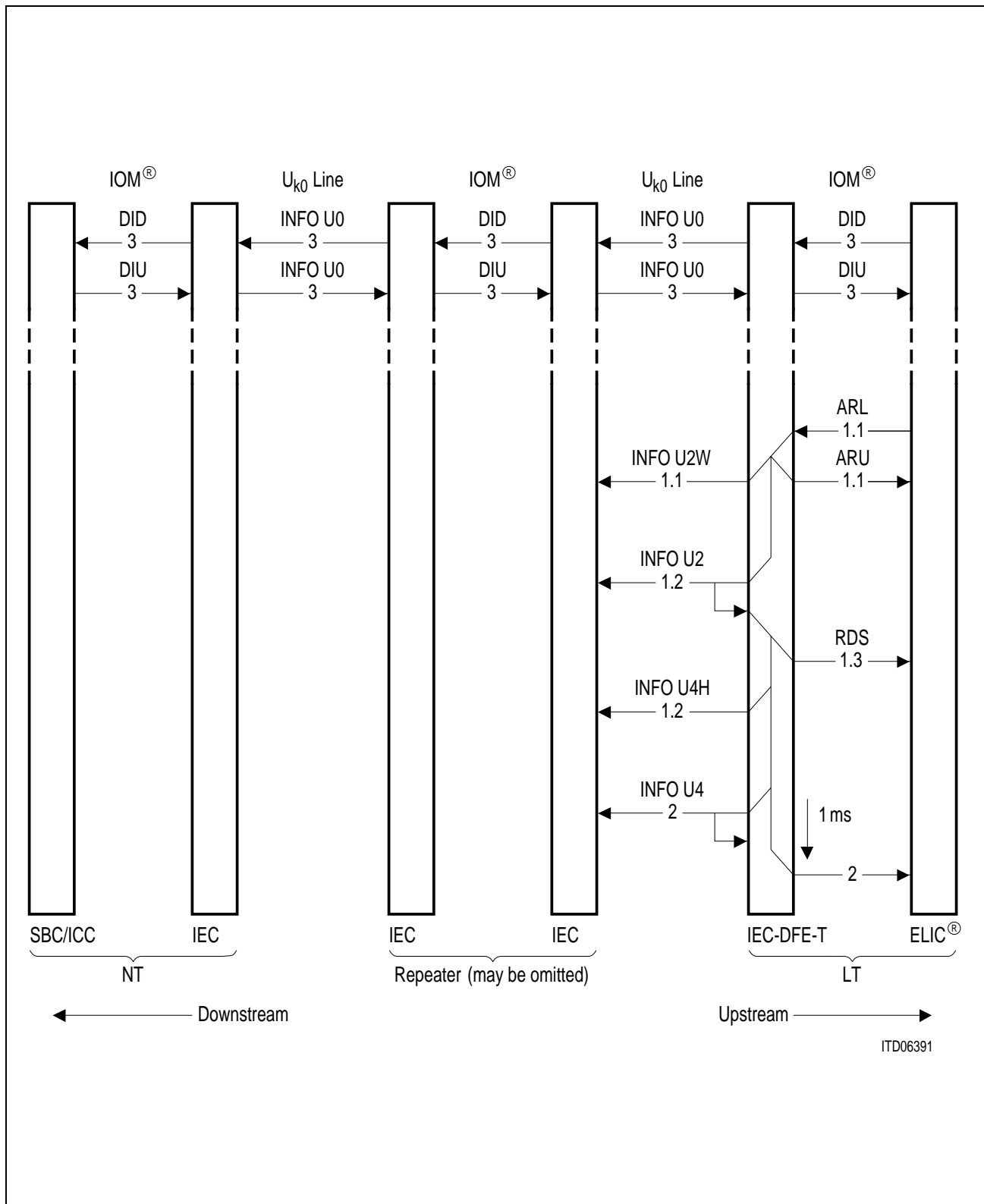
Figure 17 Activation of Loop1
