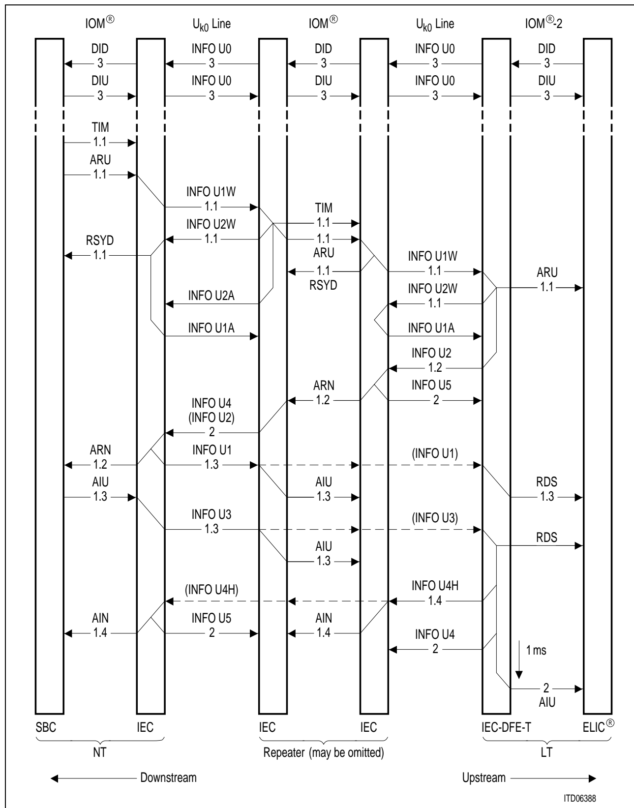
Figure 14 Activation of U_{k0} Link Initiated by NT
