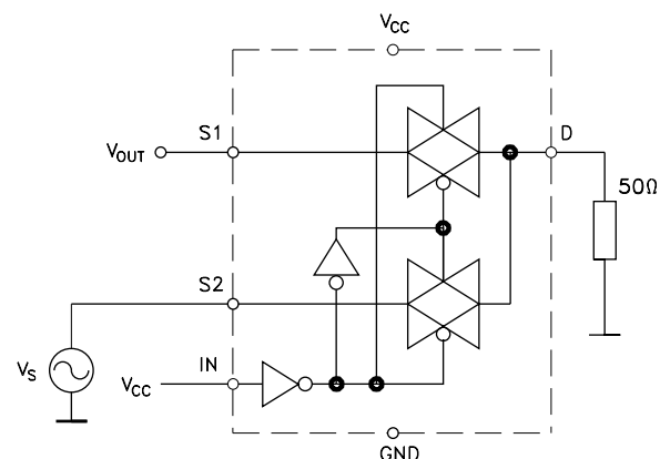
Figure 8. Channel-to-channel crosstalk
