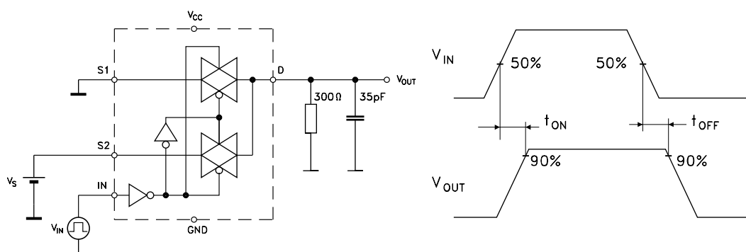
Figure 9. Switching times
