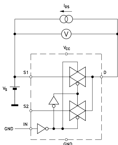
Figure 3. On-resistance
