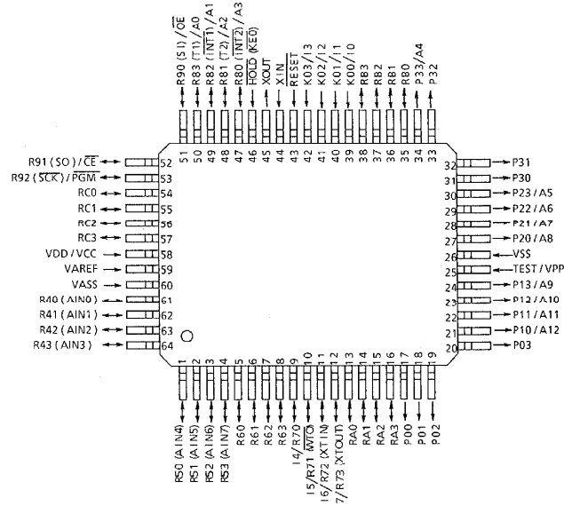
QFP64-P-1420-1.00A
