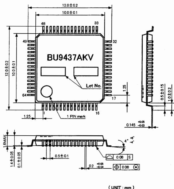
Figure 1. External dimension
