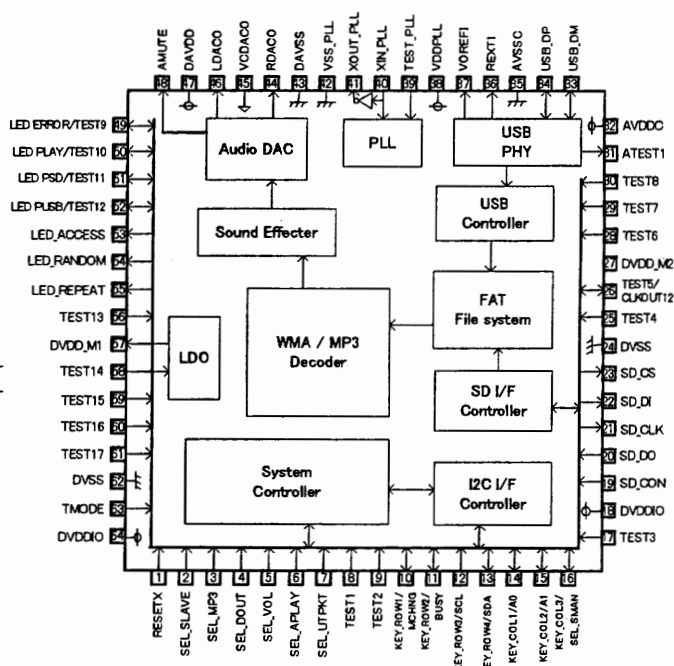
Figure 2. Block diagram
