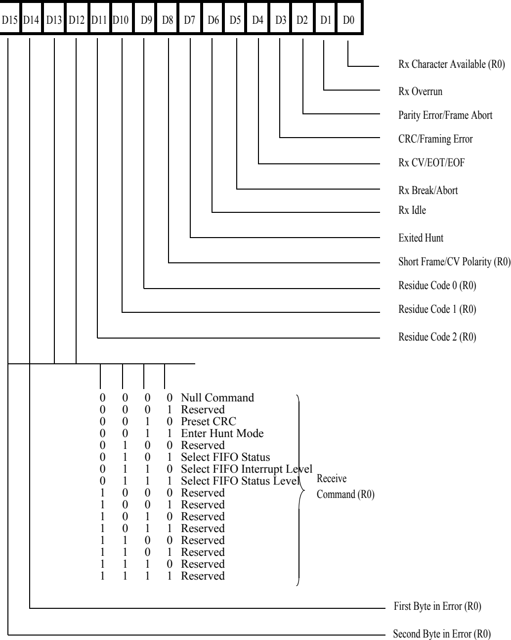
Figure 60. Receive Command Status Register
