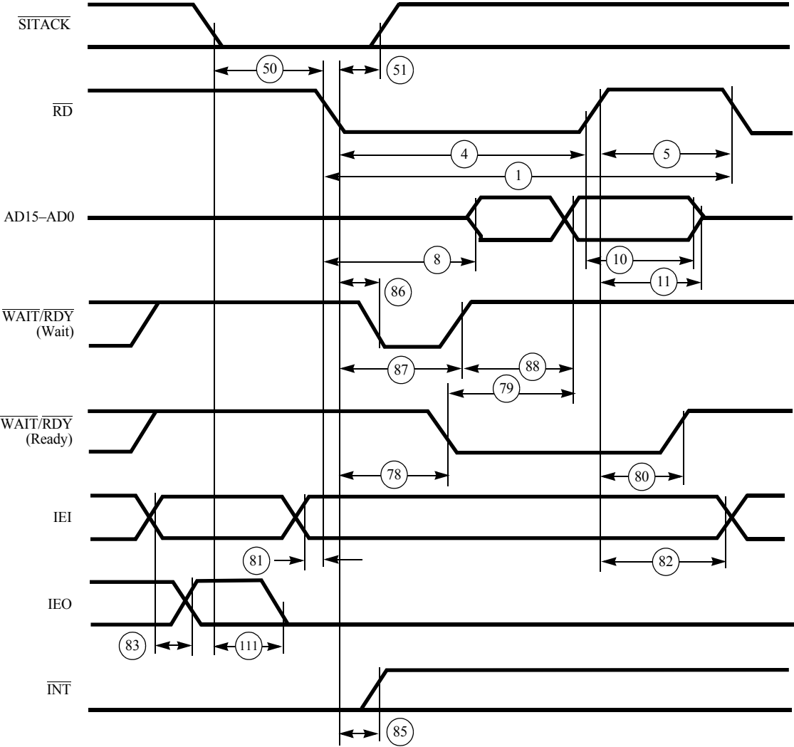
Figure 22. Nonmultiplexed \overline{\text{RD}} Interrupt Acknowledge Cycle
