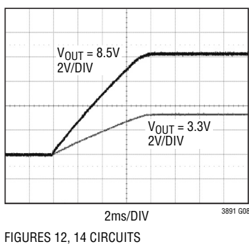
Soft Start-Up
