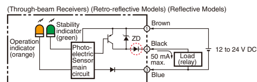
Models with PNP Output
