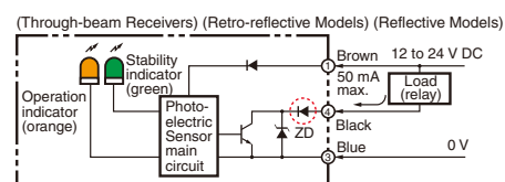
Models with NPN Output
